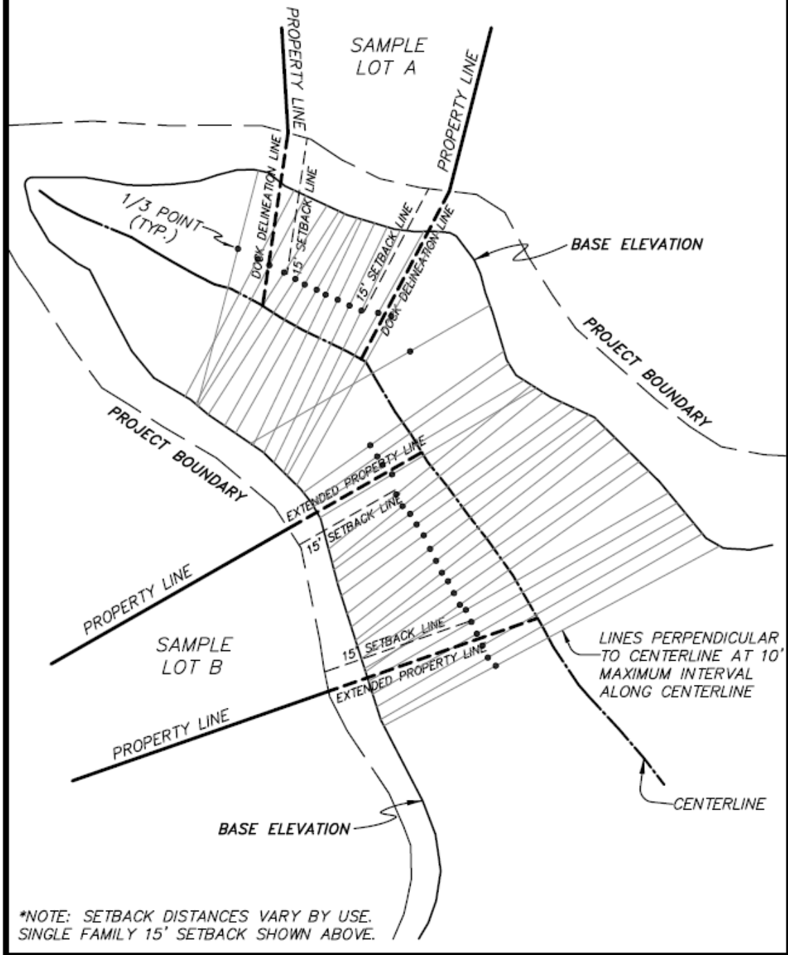
FIGURE 3 STEP THREE – DETERMINATION OF ONE-THIRD POINTS
