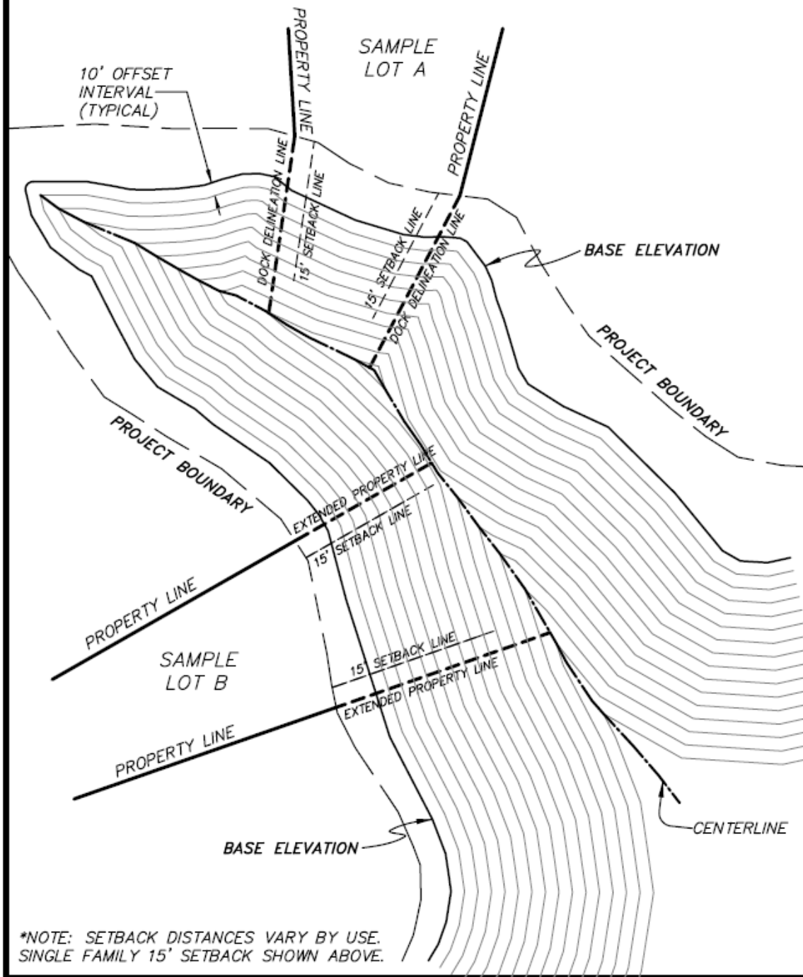
FIGURE 2 STEP TWO – DETERMINATION OF WATERWAY CENTERLINE
