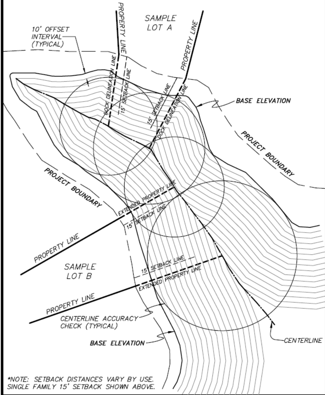
FIGURE 2A STEP TWO – DETERMINATION OF WATERWAY CENTERLINE (ACCURACY CHECK)
